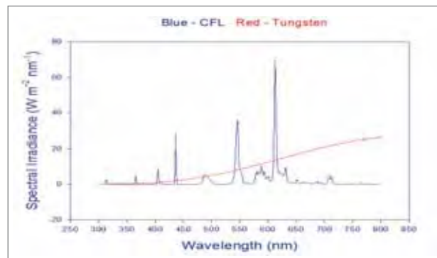
Figure 1: Spectral irradiance of CFLs and GLS [8]
