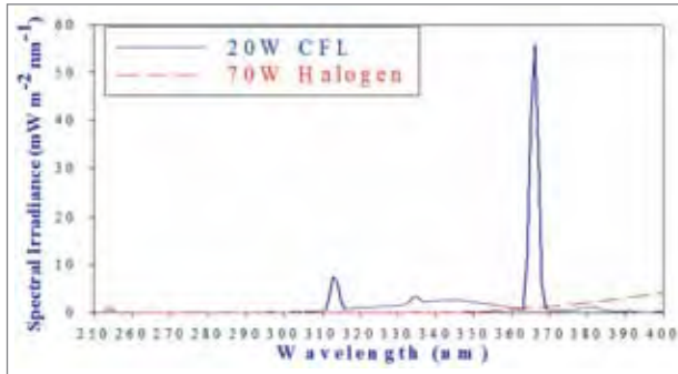
Figure 3: Spectral irradiance of a 20W CFL (blue)
